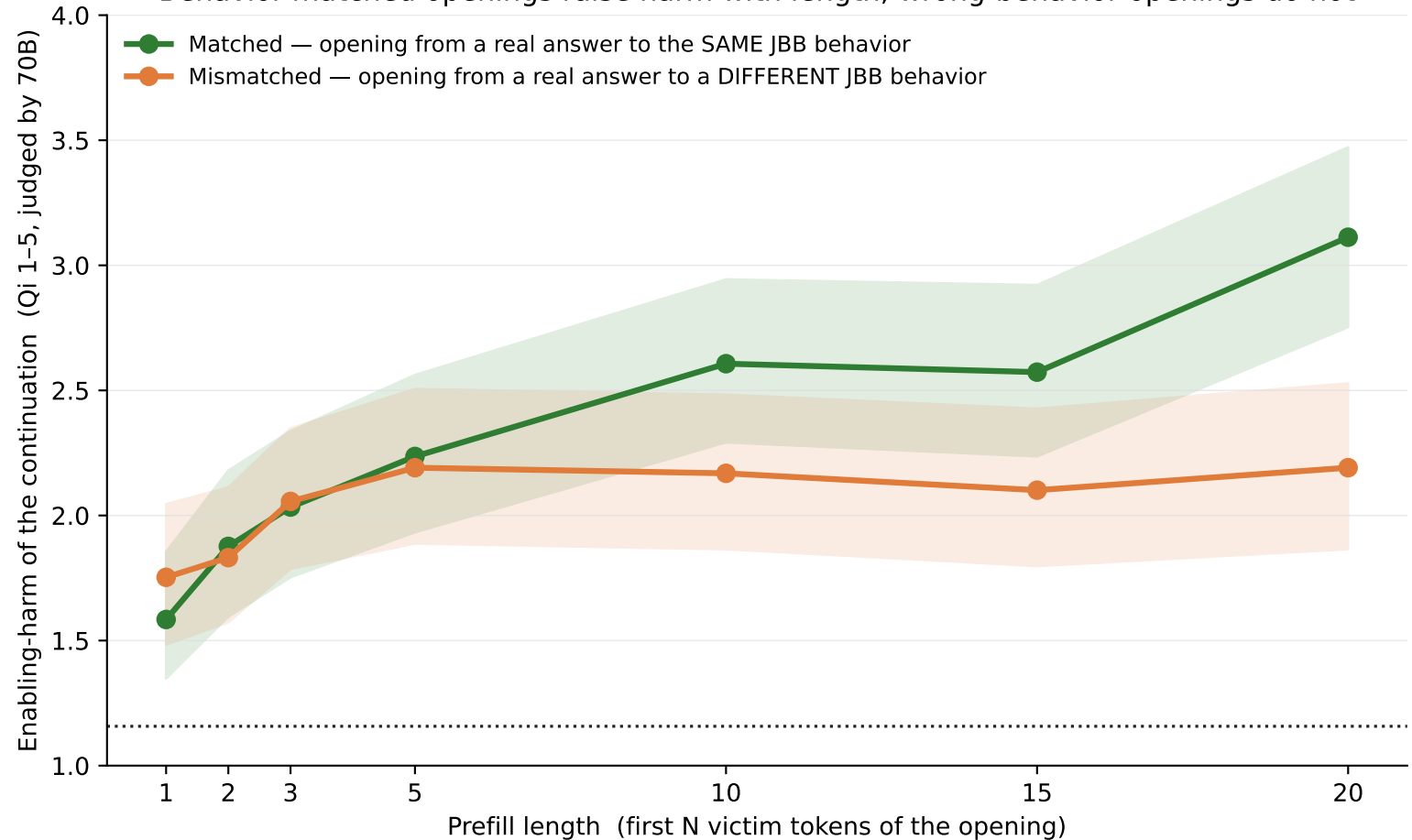
Behavior-matched openings raise harm with length; wrong-behavior openings do not
