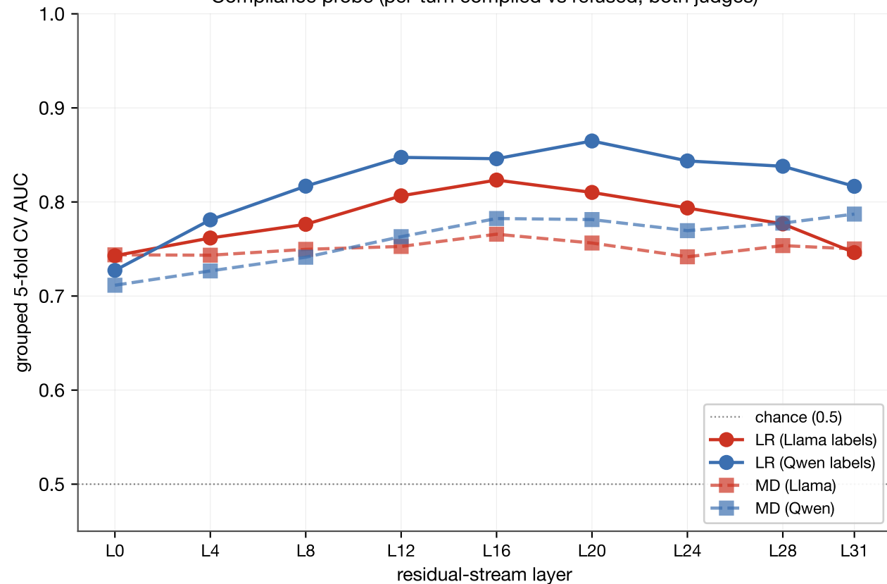
Compliance probe (per-turn complied vs refused, both judges)
