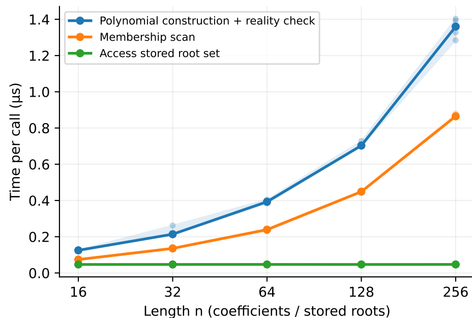
Distinct rational values 1..n
