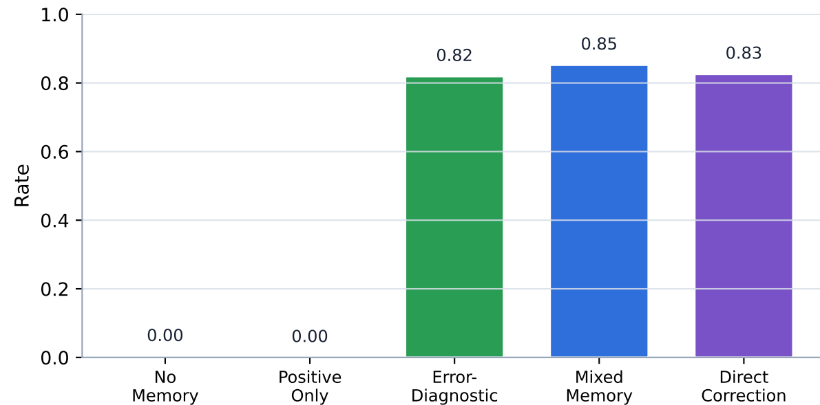
C. Cross-architecture: Correction Success
