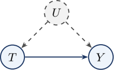
explicit U
