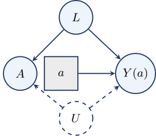
SWIG \mathcal{G}(a) (with hidden U )
