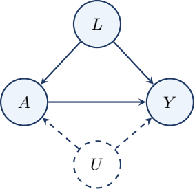
DAG (with hidden U )
