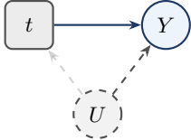
Mutilated DAG: \text{do}(T=t)
