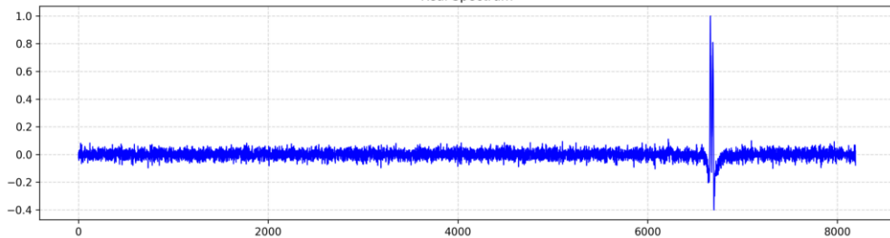
Real Spectrum
