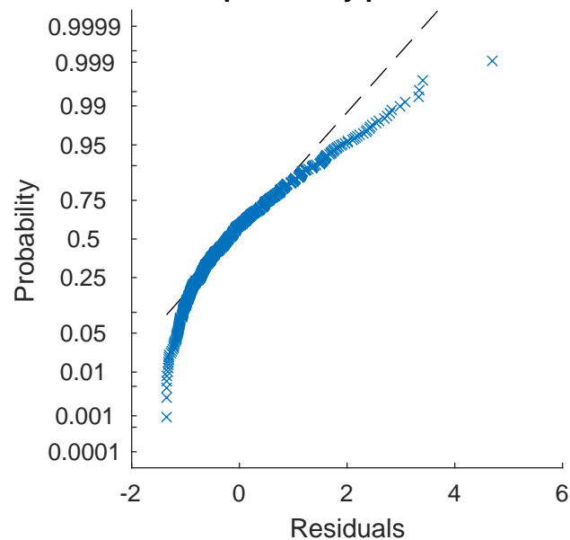
Normal probability plot of residuals
