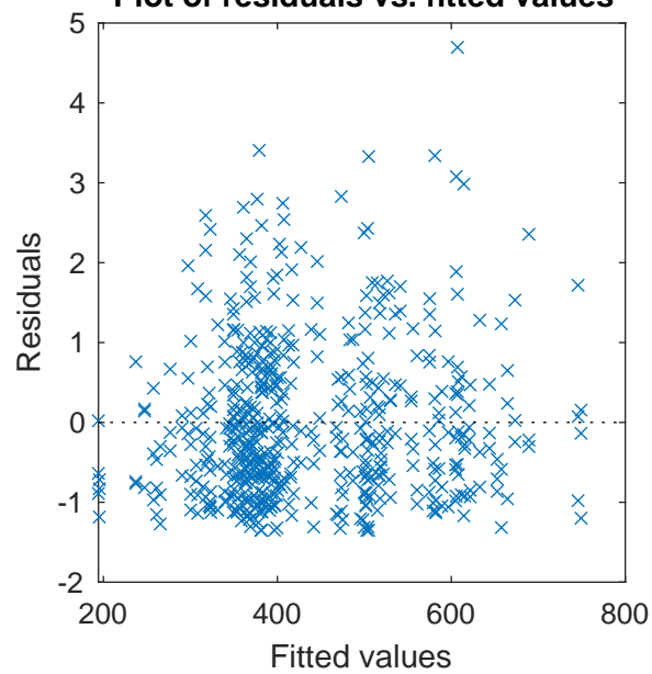
Plot of residuals vs. fitted values
