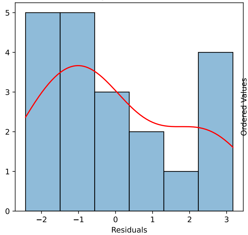
Lagged Residuals
