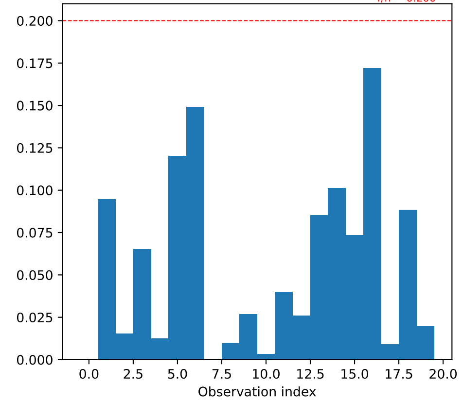
Cook's Distance
