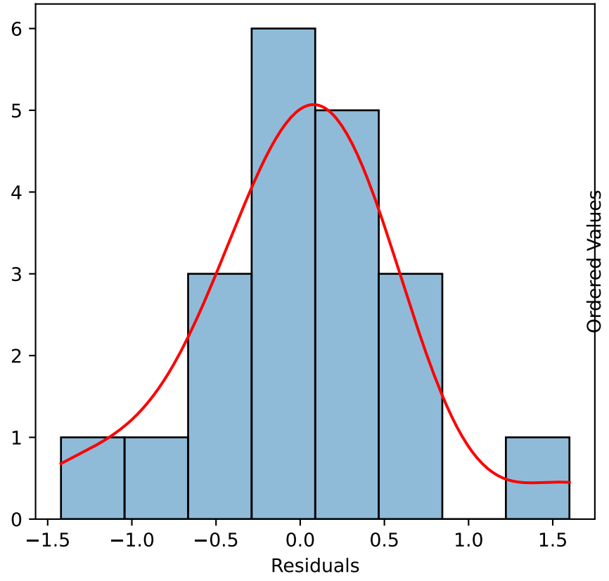
Lagged Residuals
