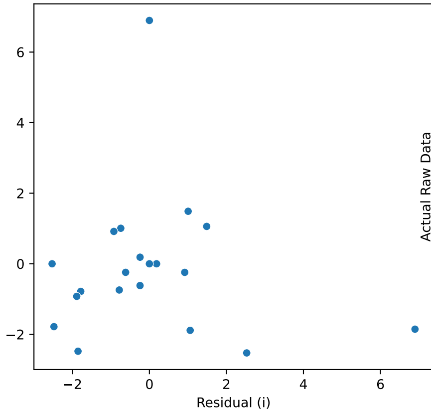
Lagged Residuals
