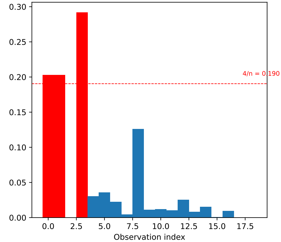
Cook's Distance
