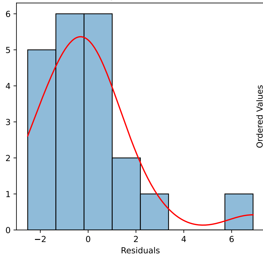
Lagged Residuals
