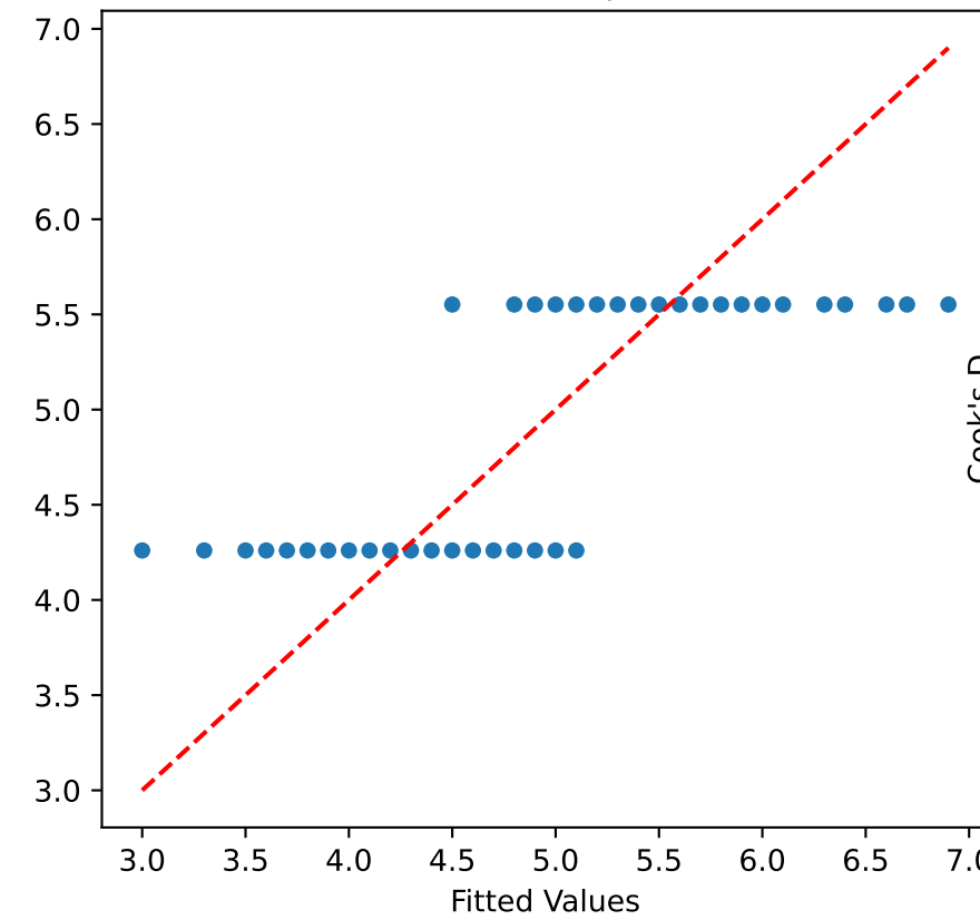
Fitted vs Response
