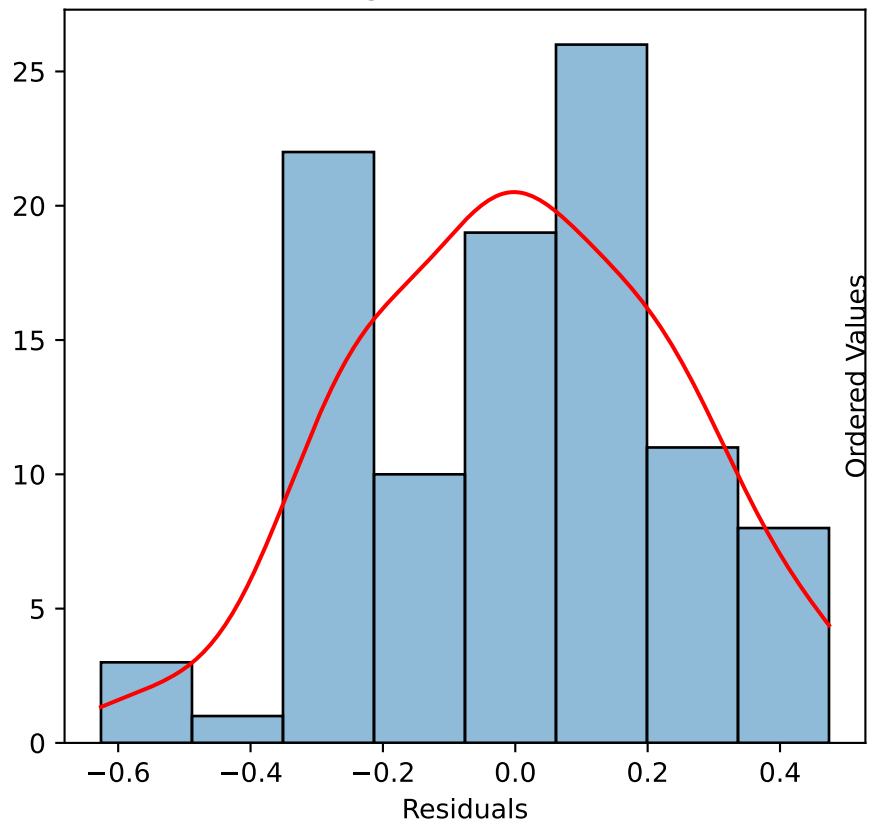
Lagged Residuals
