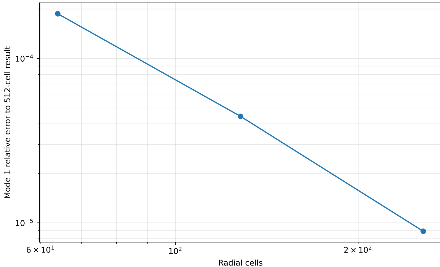
Grid-convergence diagnostic
