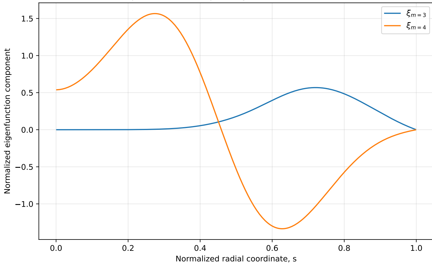
Representative coupled eigenmode 2: 271.12 kHz
