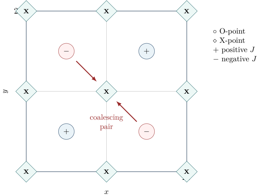
Figure 1: Topology of \psi_0 = \sin x \sin y . The stream-function perturbation drives the two negative-current islands toward the central X-point. Periodicity creates an equivalent pairing of the positive-current islands across the domain boundary. The drawing identifies critical points; it is not a computed trajectory.
