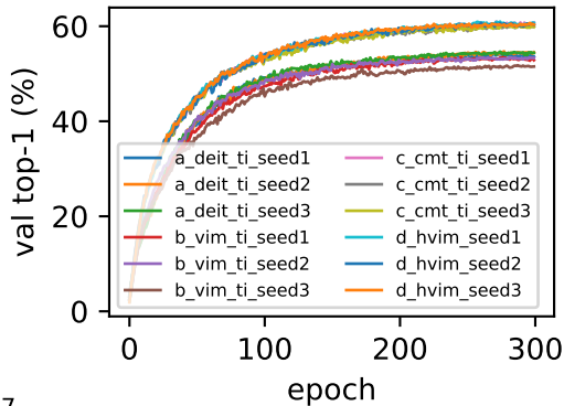
Validation curves
