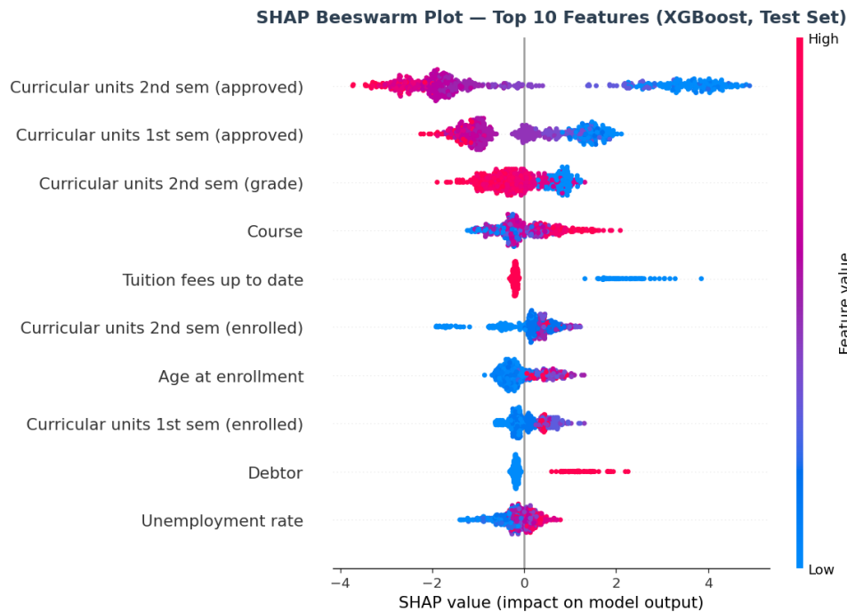
Figure 5: SHAP Beeswarm Plot — Top 10 Features (XGBoost, Test Set). Each dot represents one student. Colour indicates feature value (red = high, blue = low).
