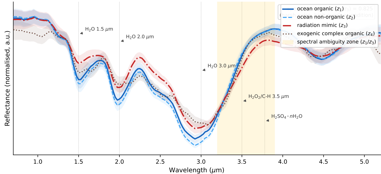
Fig. 2 — Representative synthetic spectra by hidden source class (mean \pm 1\sigma over 40 realisations, moderate noise)
