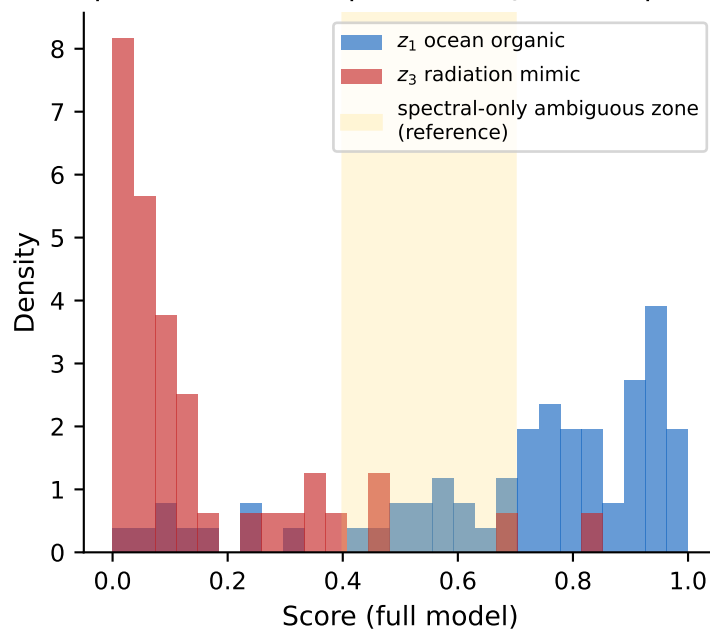
(B) Full model — ambiguous-subset samples re-scored (spatial context disperses z_1/z_3 toward poles)
