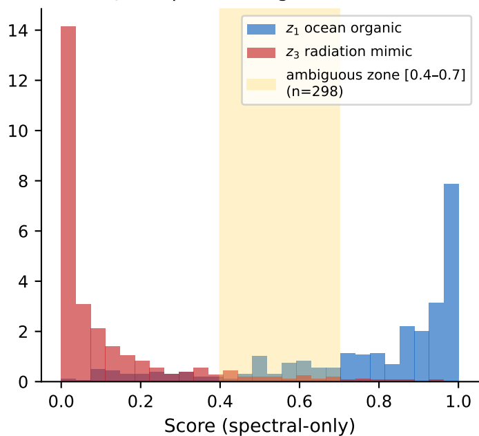
(A) Spectral-only — full score distribution (all z_1/z_3 samples; ambiguous zone shaded)
