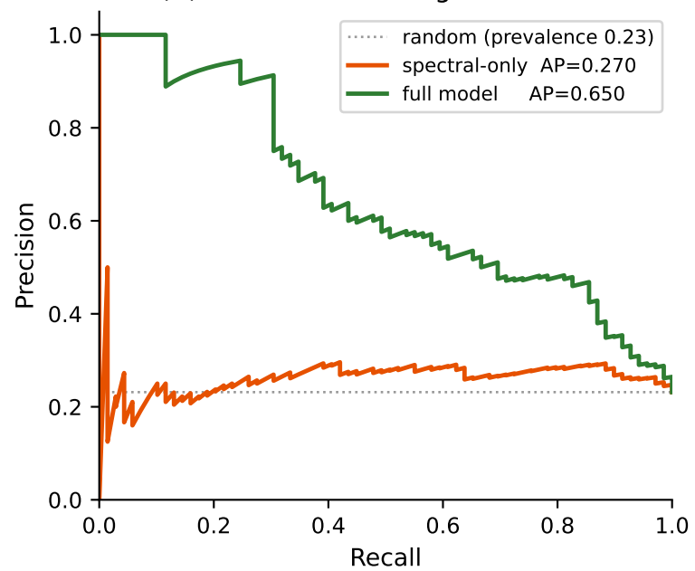
(C) PR curve — ambiguous subset
