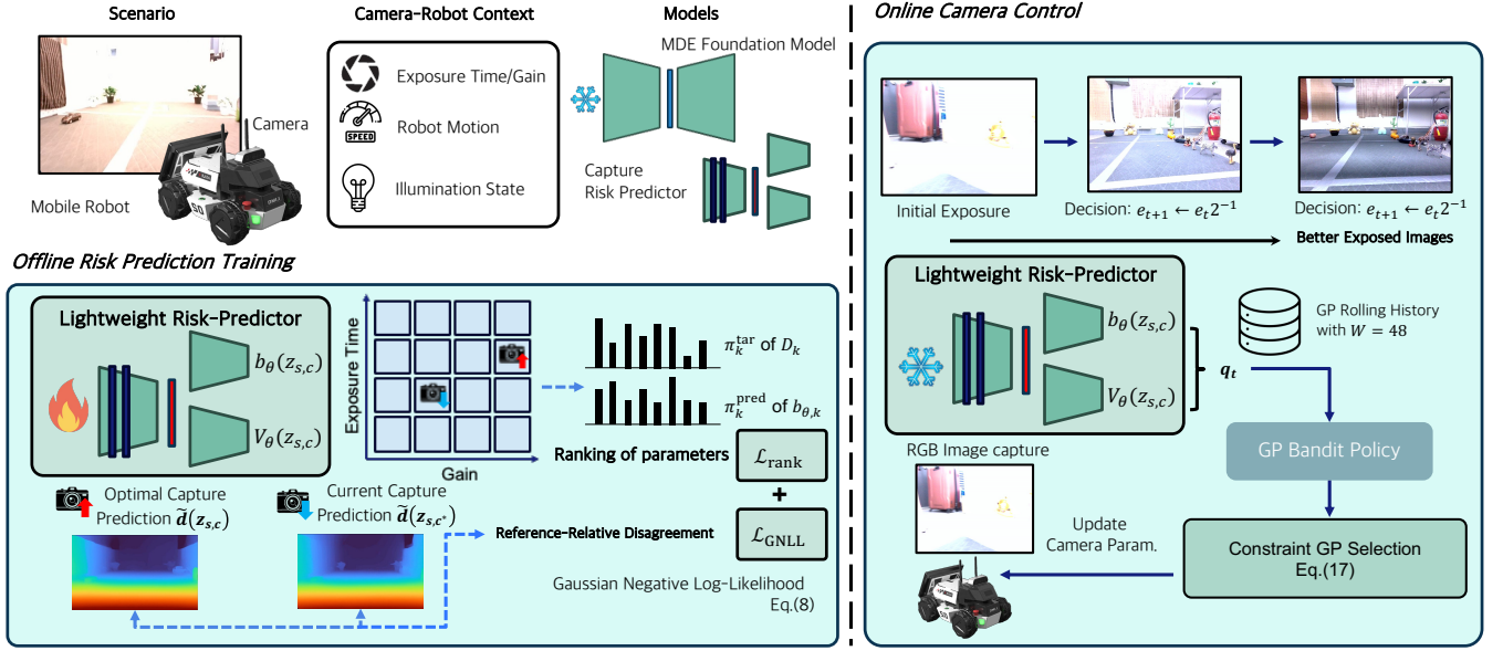
Fig. 2: A lightweight FiLM [30]-conditioned network uses frozen MDE features with camera, motion, and illumination information to predict the mean and variance of reference-relative prediction disagreement. The target is constructed using the best evaluated reference capture and optimized using Gaussian negative log-likelihood and ranking losses.
