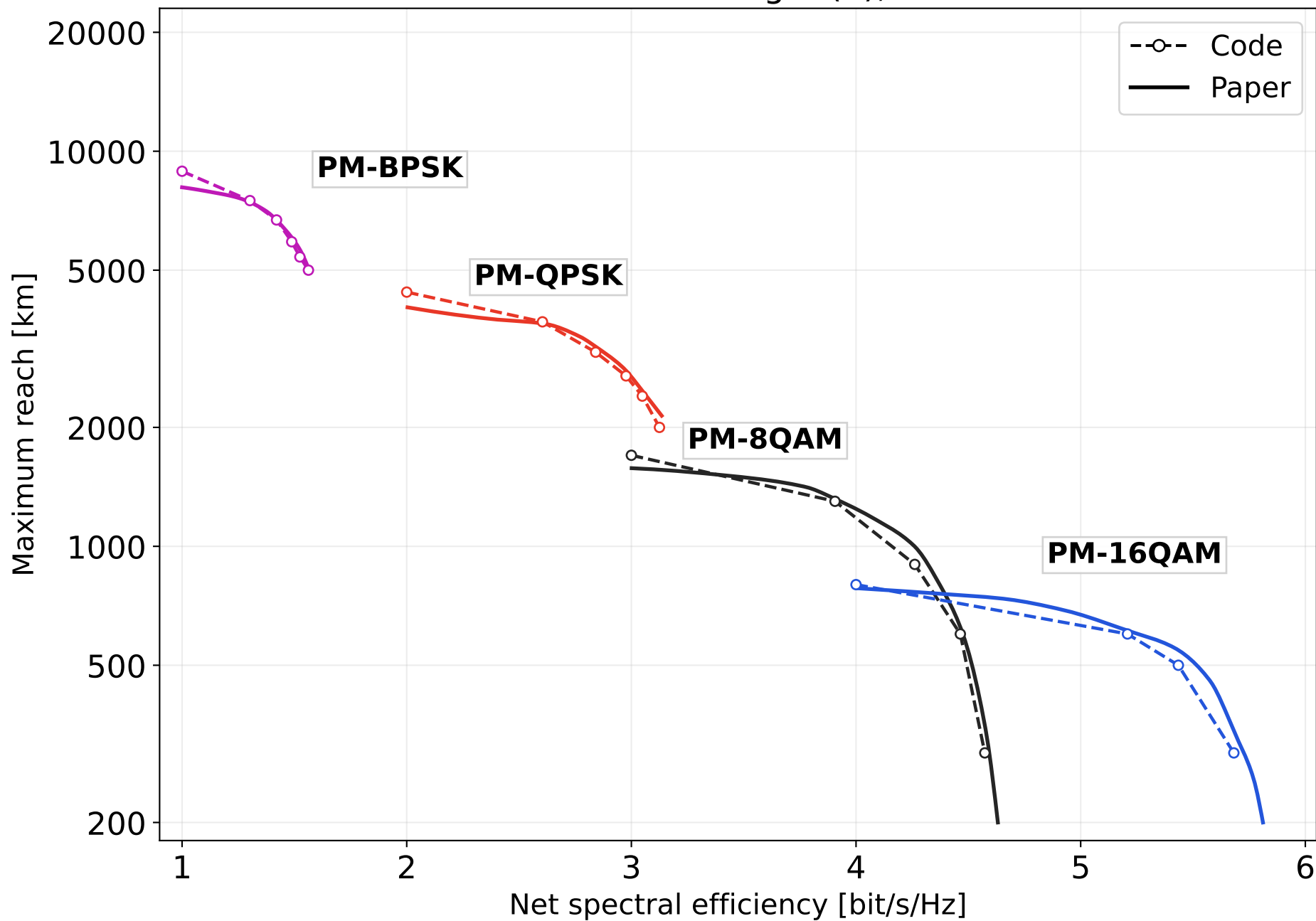
Carena et al. Fig. 5(b), SMF
