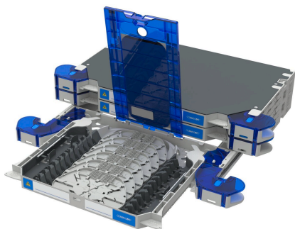
FACT® Fiber Optic Splice Chassis for FACT ODF
