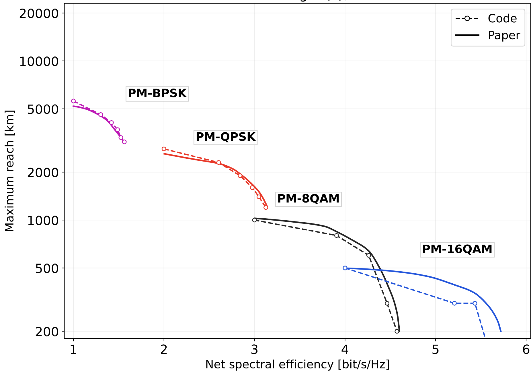
Carena et al. Fig. 5(c), NZDSF
