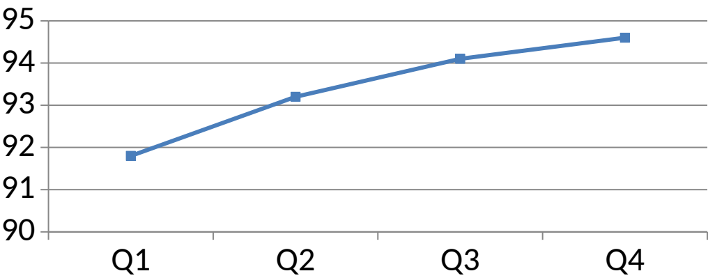
Quarterly retention
