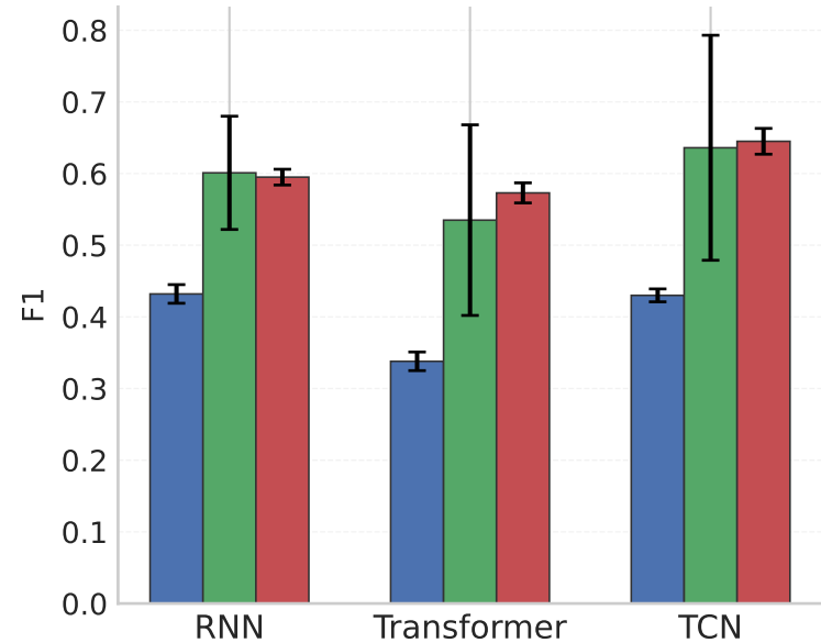
SeqCombSingle
