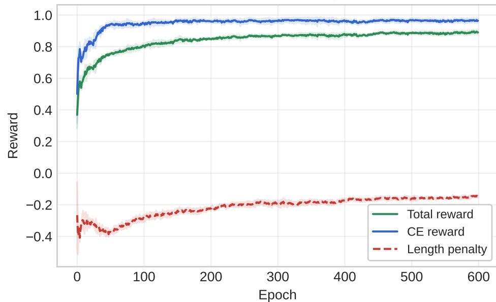
(c) Valid reward decomposition
