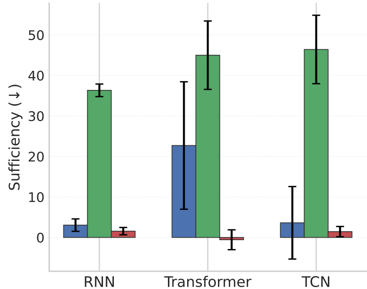
GunPoint
