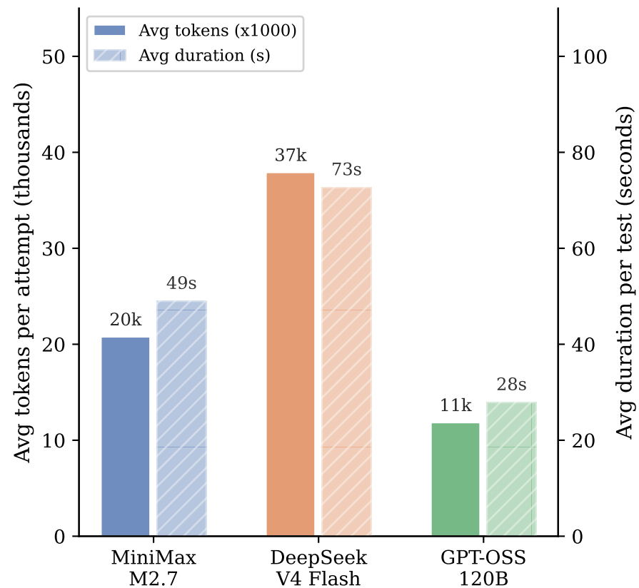
Repair Efficiency per Model
