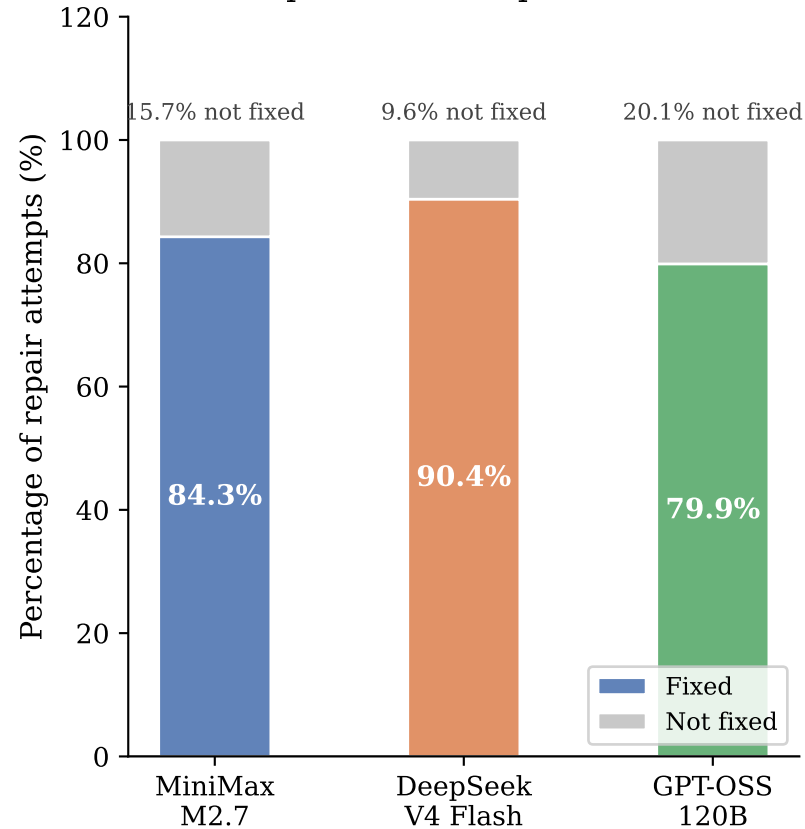
Repair Outcome per Model
