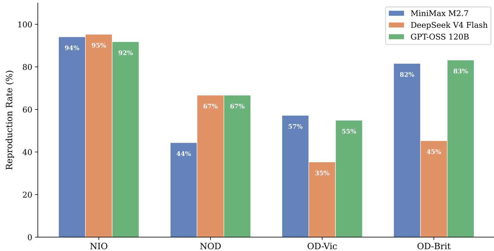
Reproduction Rate by Flaky Category and Model
