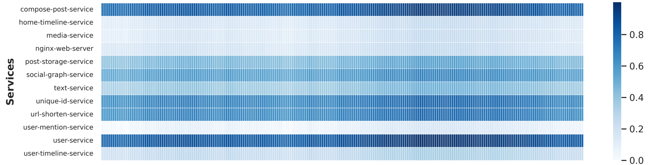
Log Attribution
