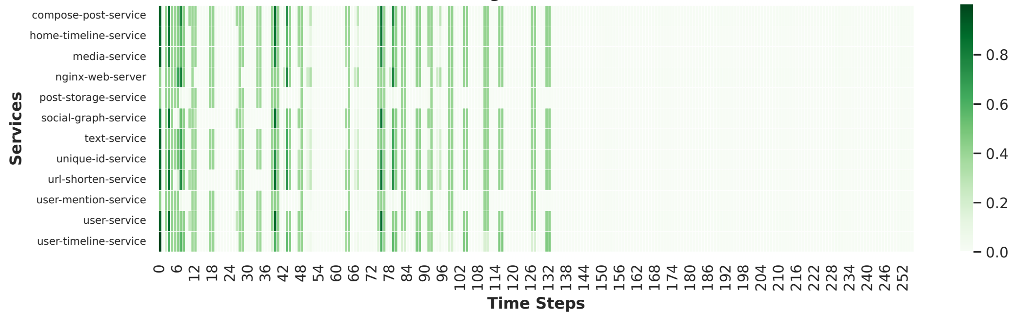
Log Attribution
