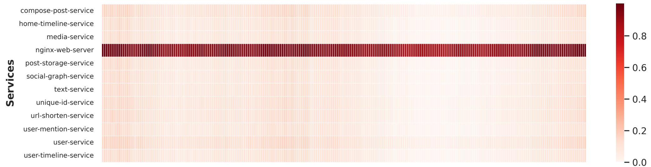
Trace Attribution
