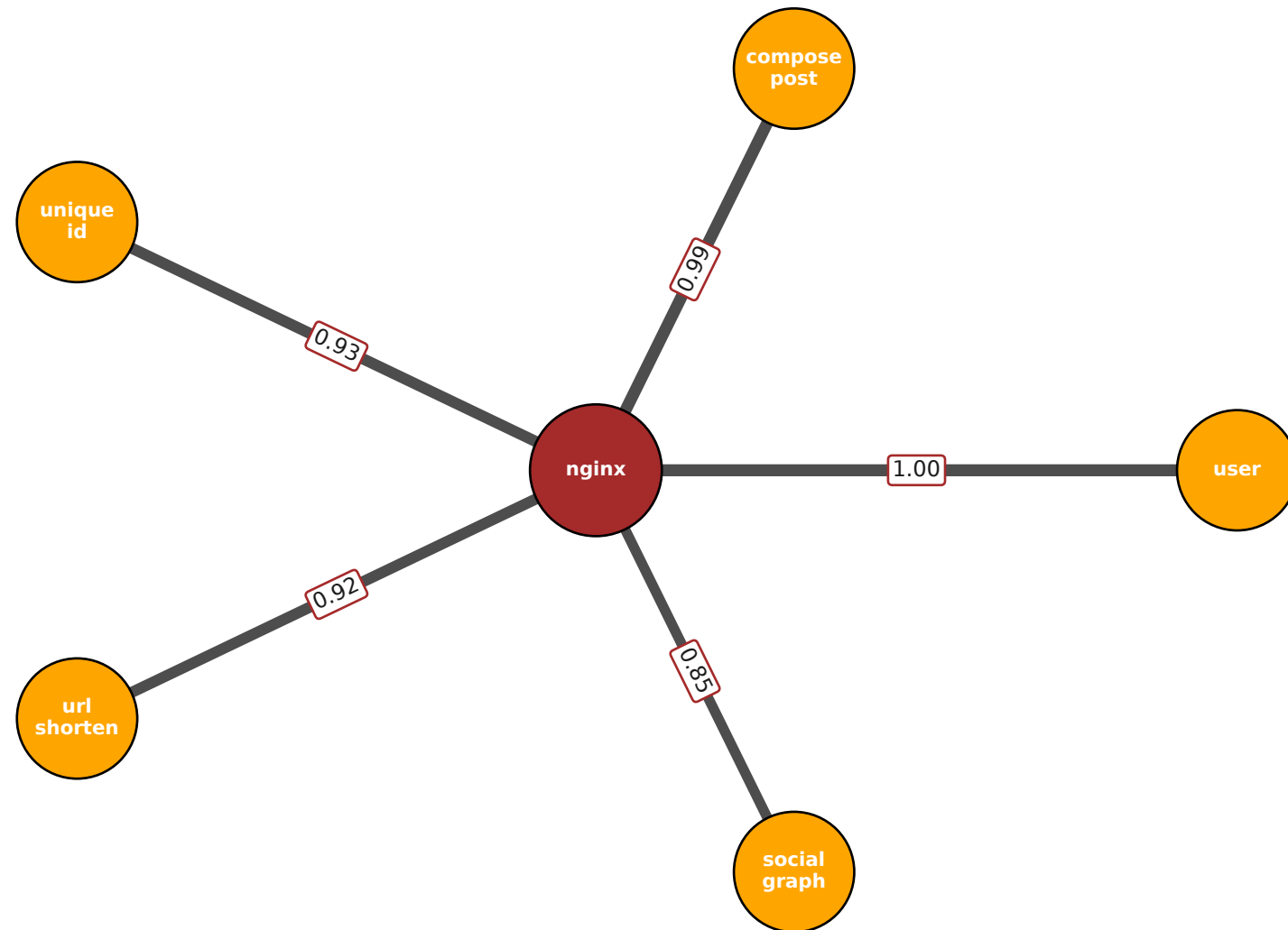
(C) Deep Backend Logic Target: social-graph-service
