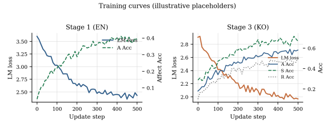
Fig. 8. Stage 1 (EN) and Stage 3 (KO) training curves.
