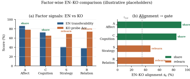
Fig. 4. Factor-wise EN-KO comparison motivating Stage 2 gates. (a) KO probe Acc for A/S/R under the Stage 1 encoder. (b) Scores s_k mapped to share/relearn/suppress (Table II).
