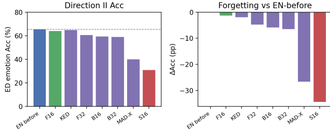
Fig. 6. Direction II return-to-EN Acc and ΔAcc (Table VII).
