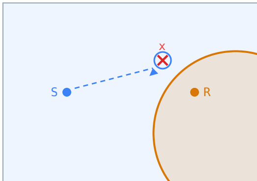
false center
