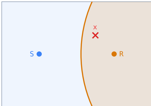
truthful
