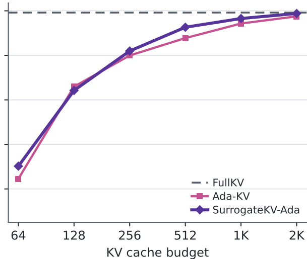
Head-aware budget
