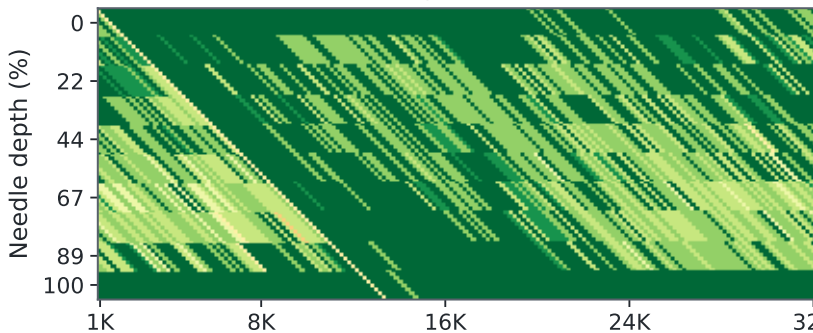
DynamicKV Avg. 98.46
