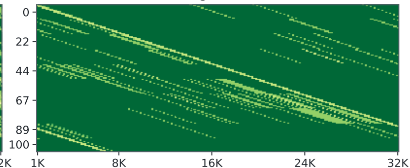
SurrogateKV-Ada Avg. 98.18
