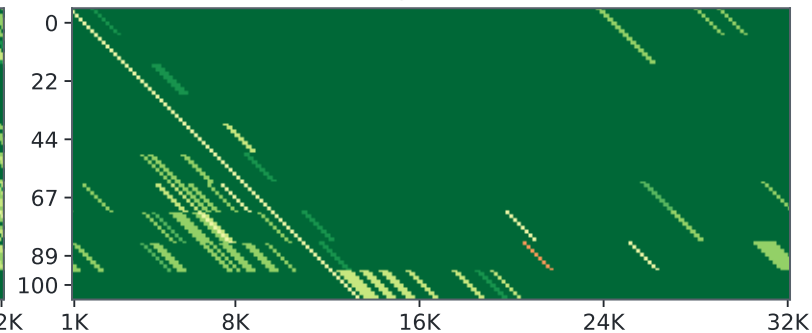
SurrogateKV-Dynamic Avg. 98.74
