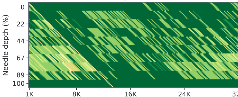
Ada-KV Avg. 90.04
