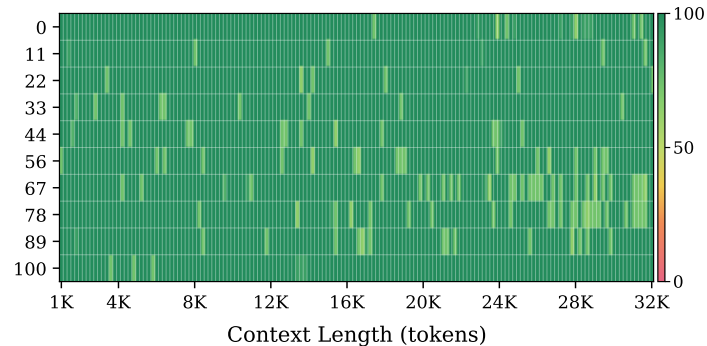
SurrogateKV-Ada (corrected)
