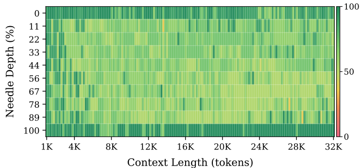
Ada-KV
