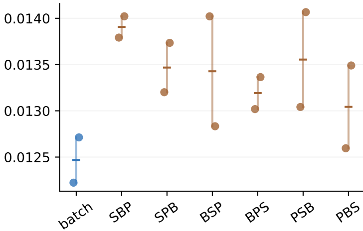
Interior high-pass MAE (lower)
