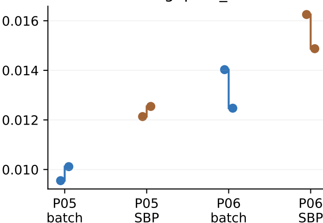
skin highpass_mae
