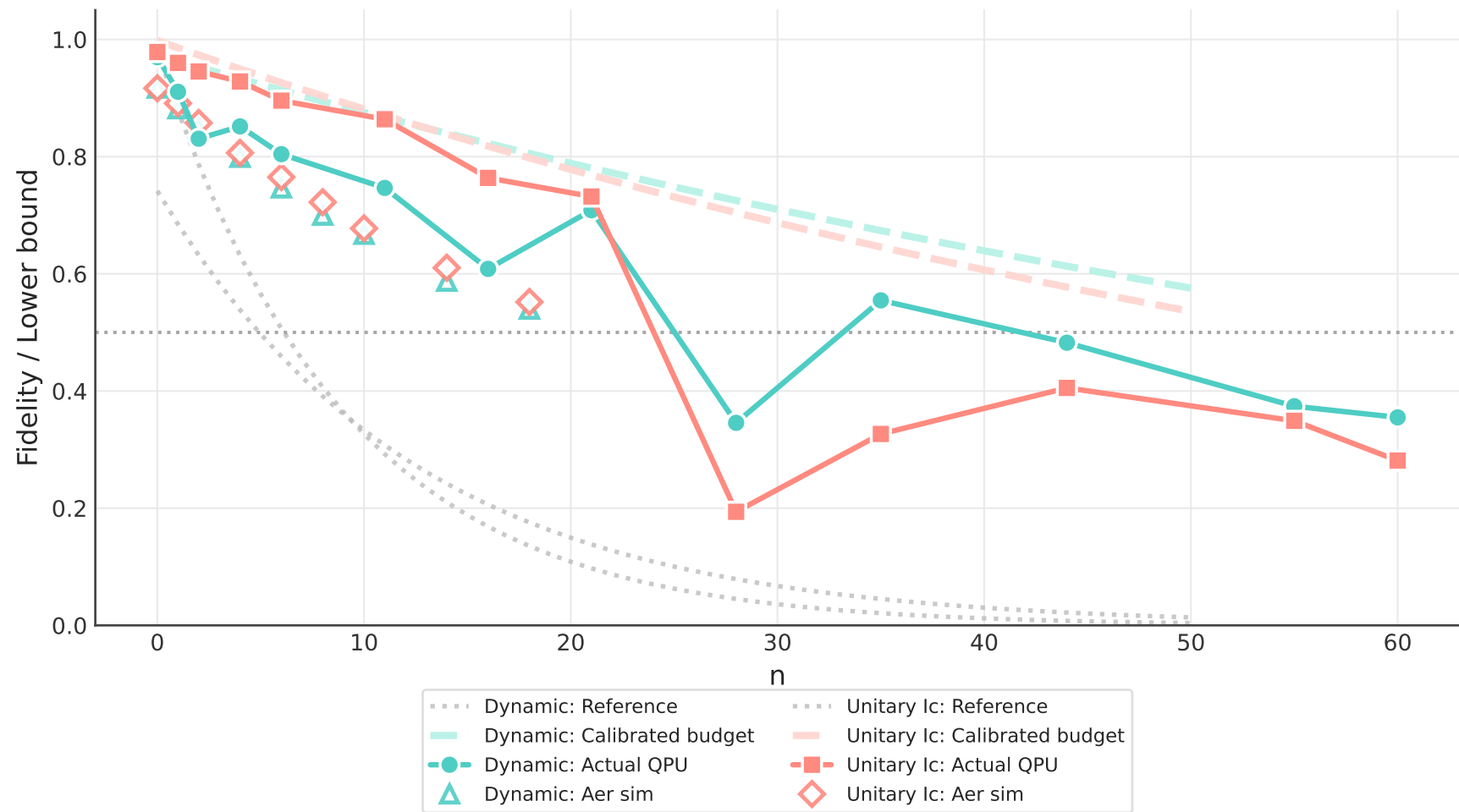
Least-Busy Actual Hardware Comparison (ibm_aachen)
