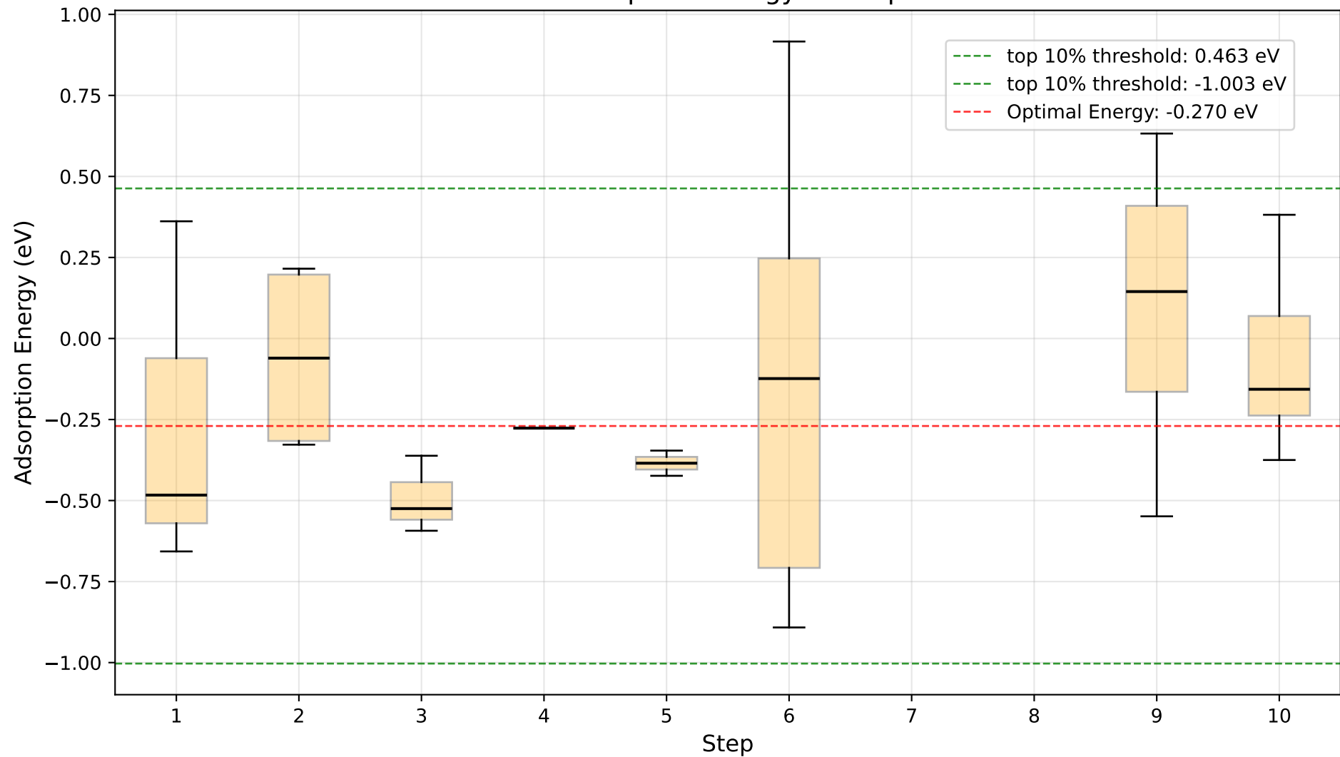
Adsorption Energy vs Step
