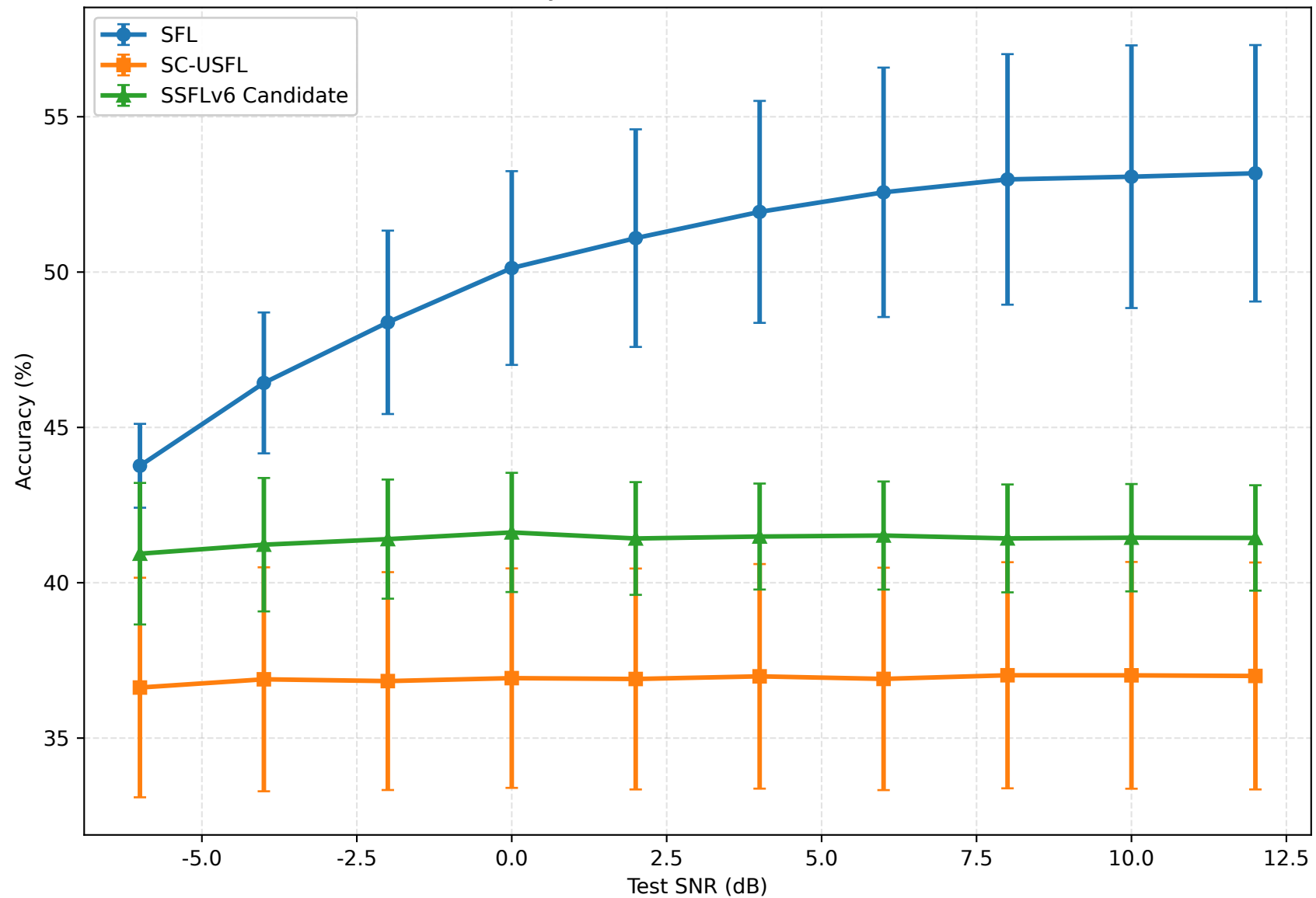
AWGN: Accuracy vs Test SNR (mean \pm std, seeds 1-4)
