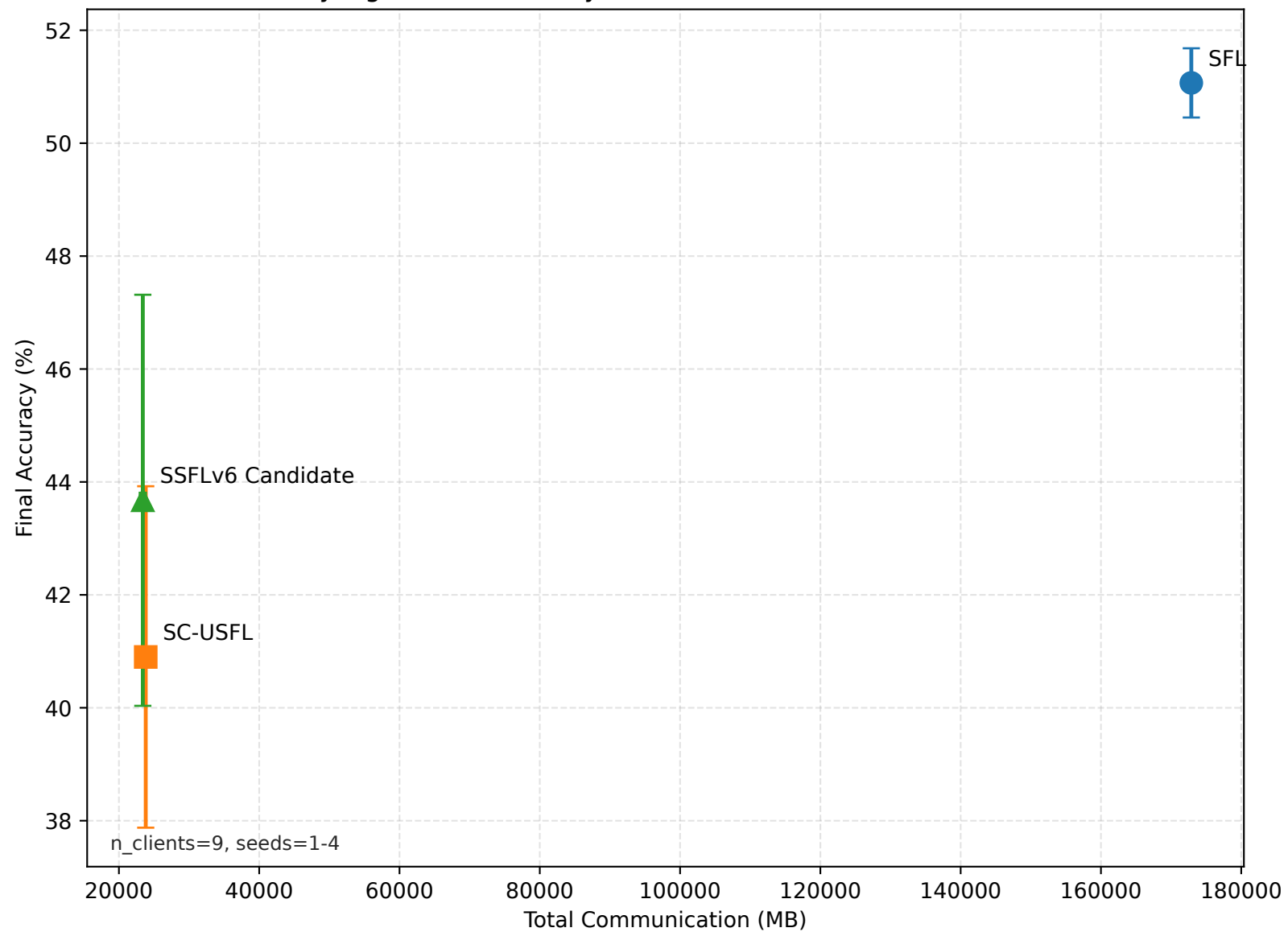
Rayleigh: Final Accuracy vs Communication (mean \pm std)
