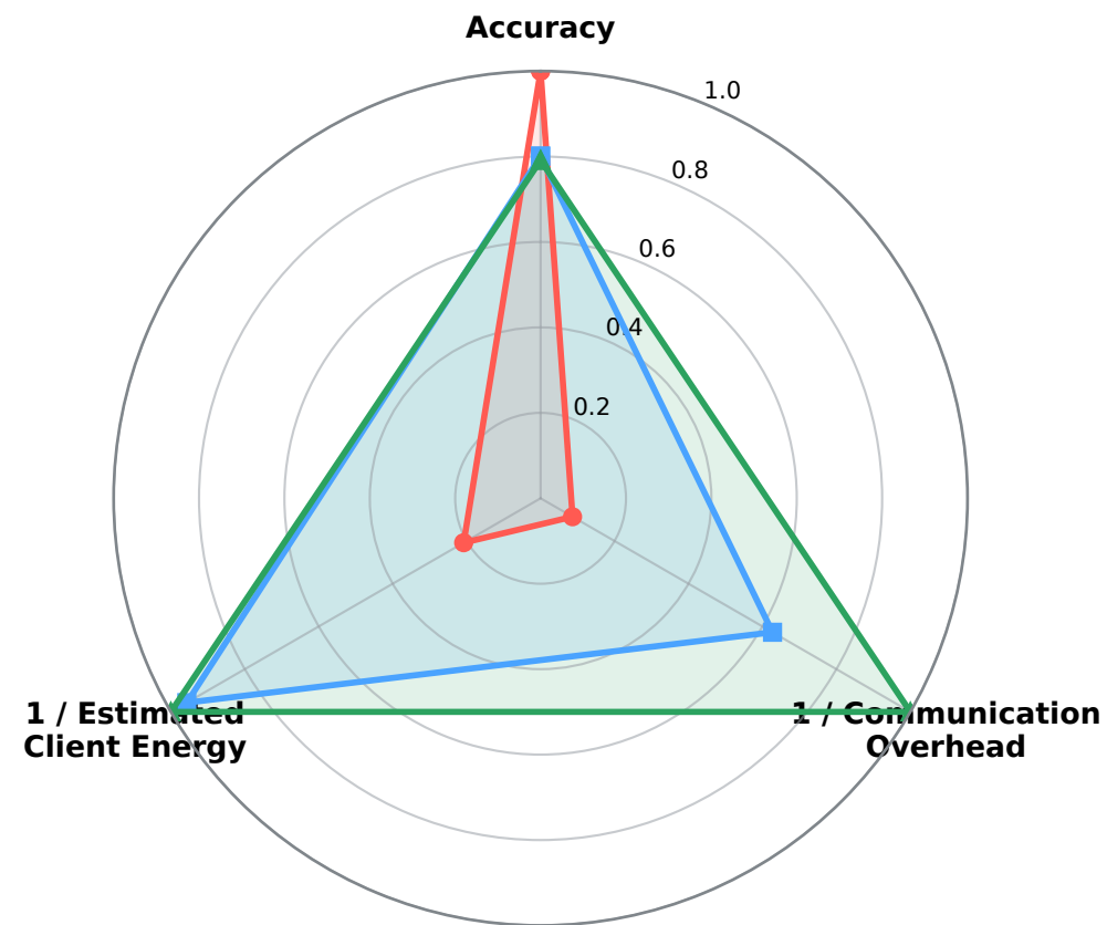
CIFAR-100 Rayleigh
