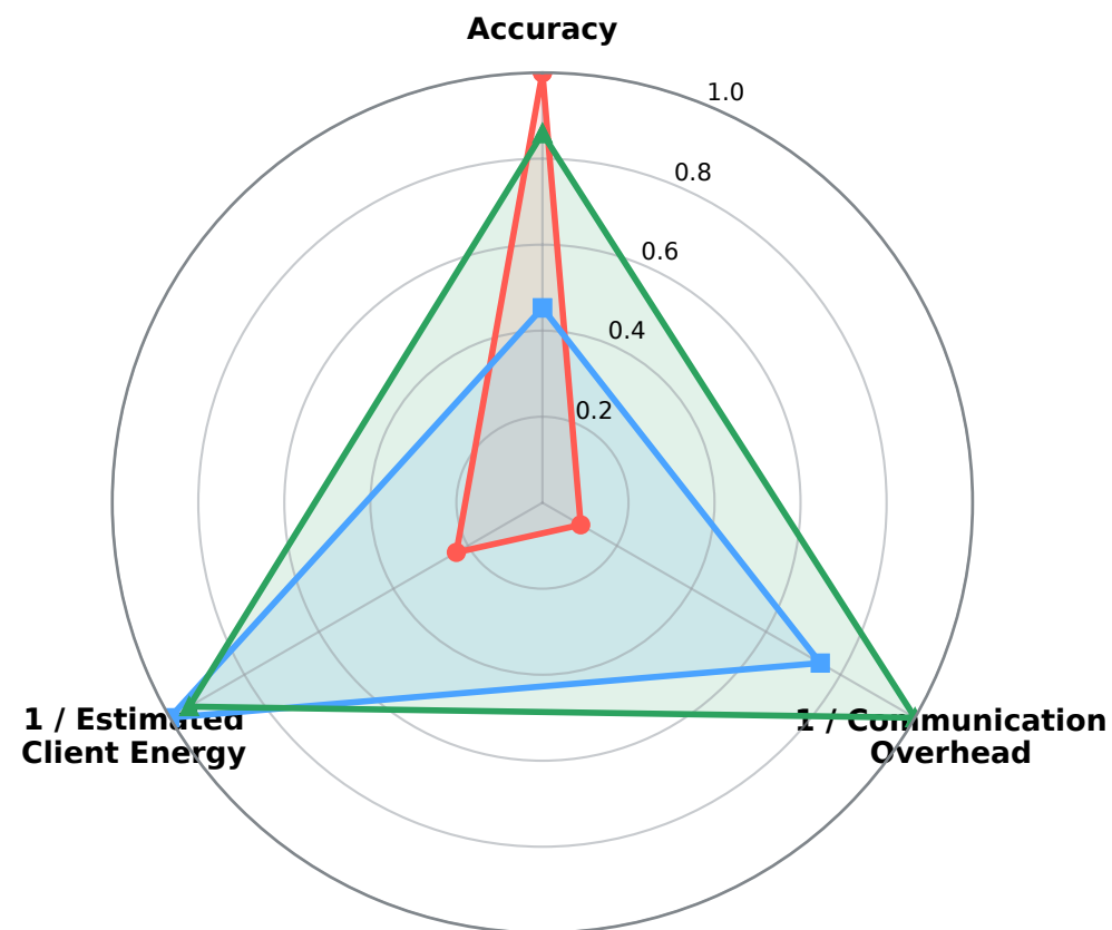
CIFAR-100 AWGN
