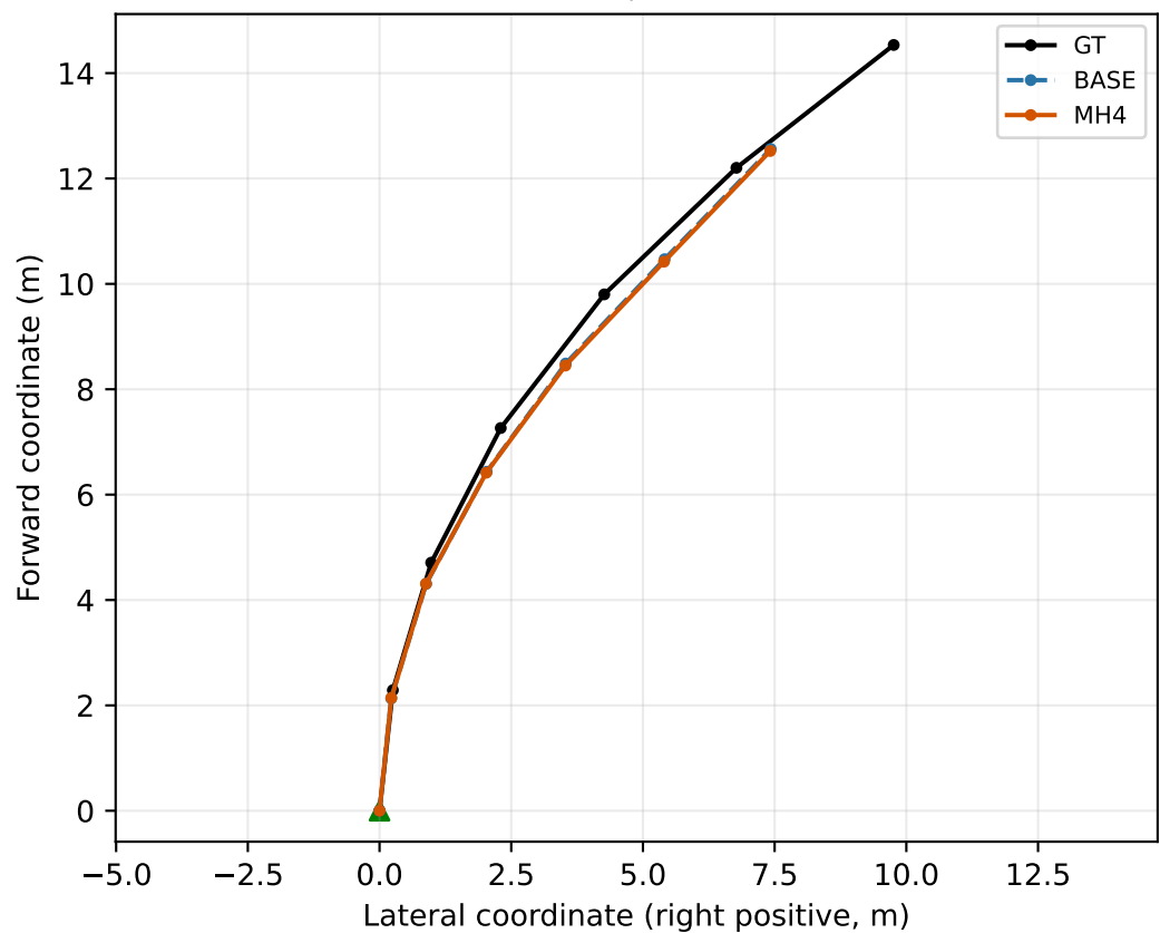
TURN_RIGHT, largest error: MH4 PREFIX 0.806 row 41690, frame 290
