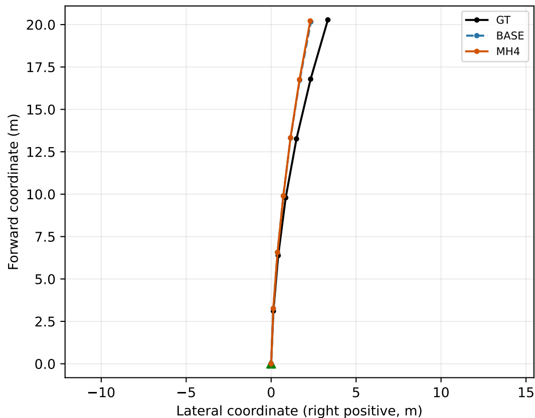
TURN_RIGHT, largest error: MH4 PREFIX 0.806 row 41690, frame 290
