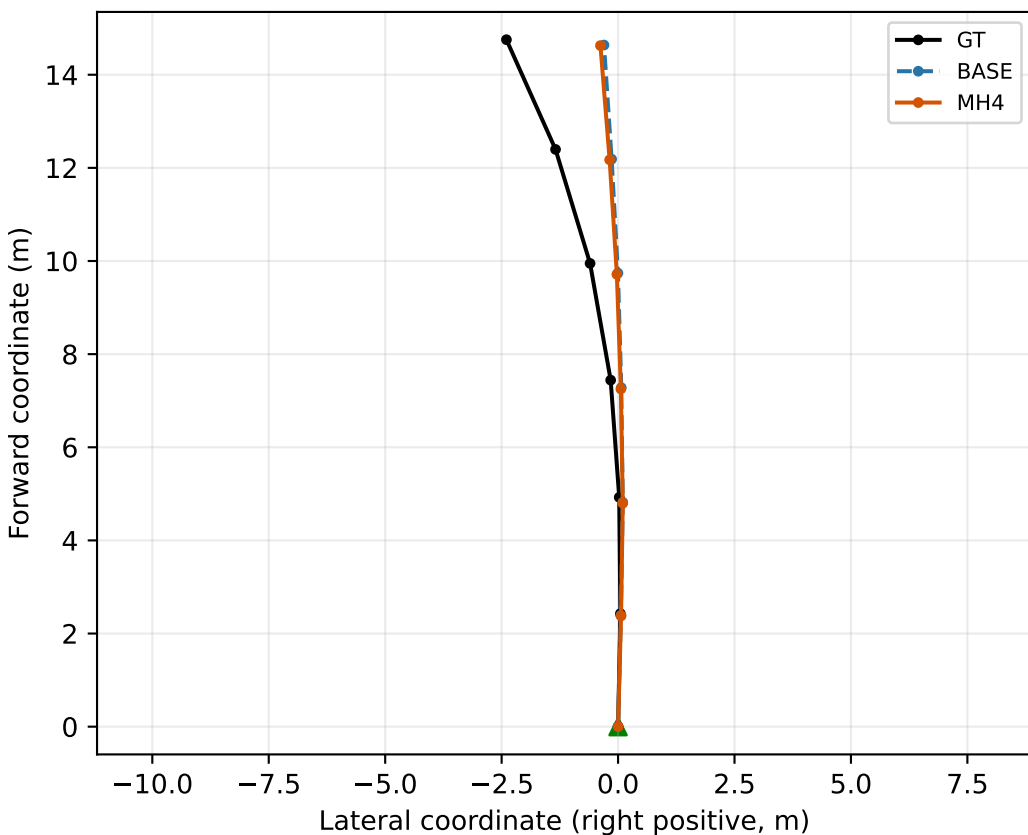
TURN_LEFT, largest error: MH4 PREFIX 0.649 row 94655, frame 155
