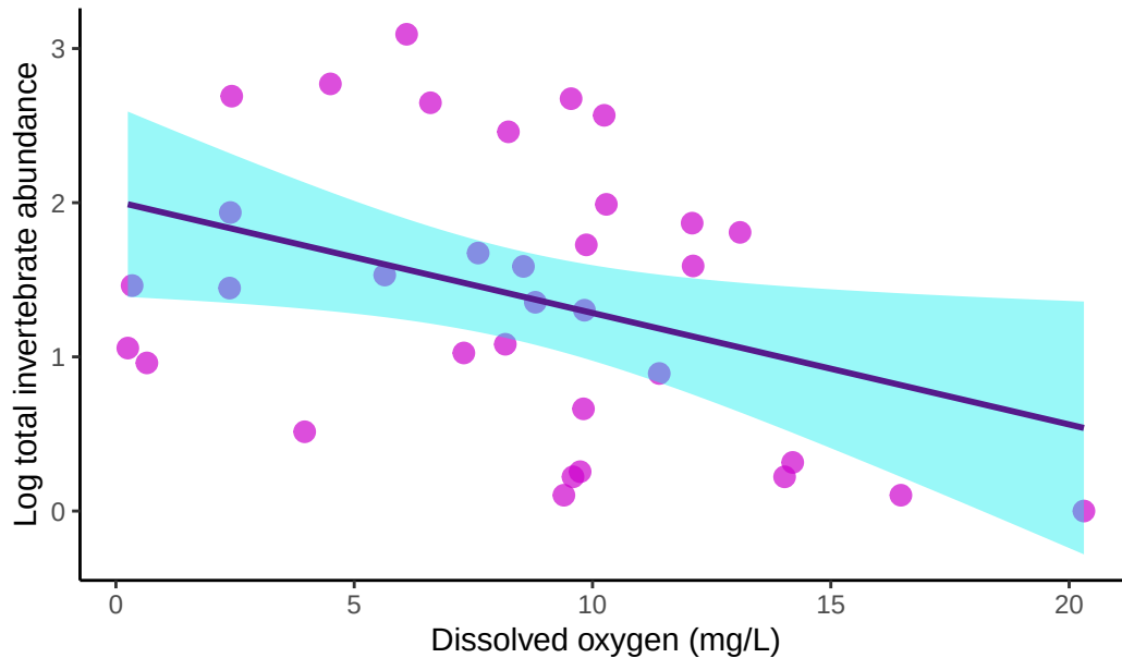
Relationship between dissolved oxygen and total invertebrate abundance
