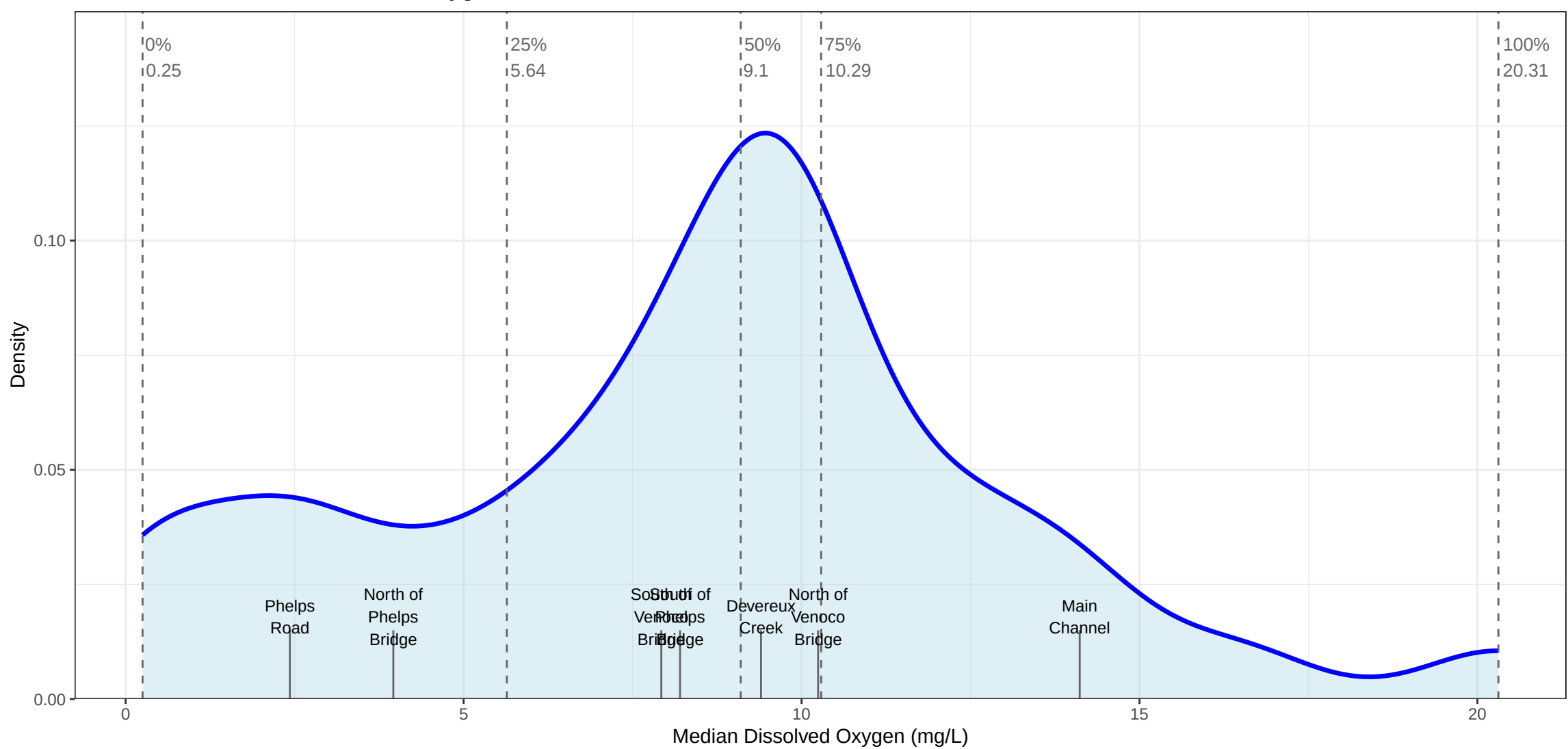
Distribution of Median Dissolved Oxygen Aross Sites
