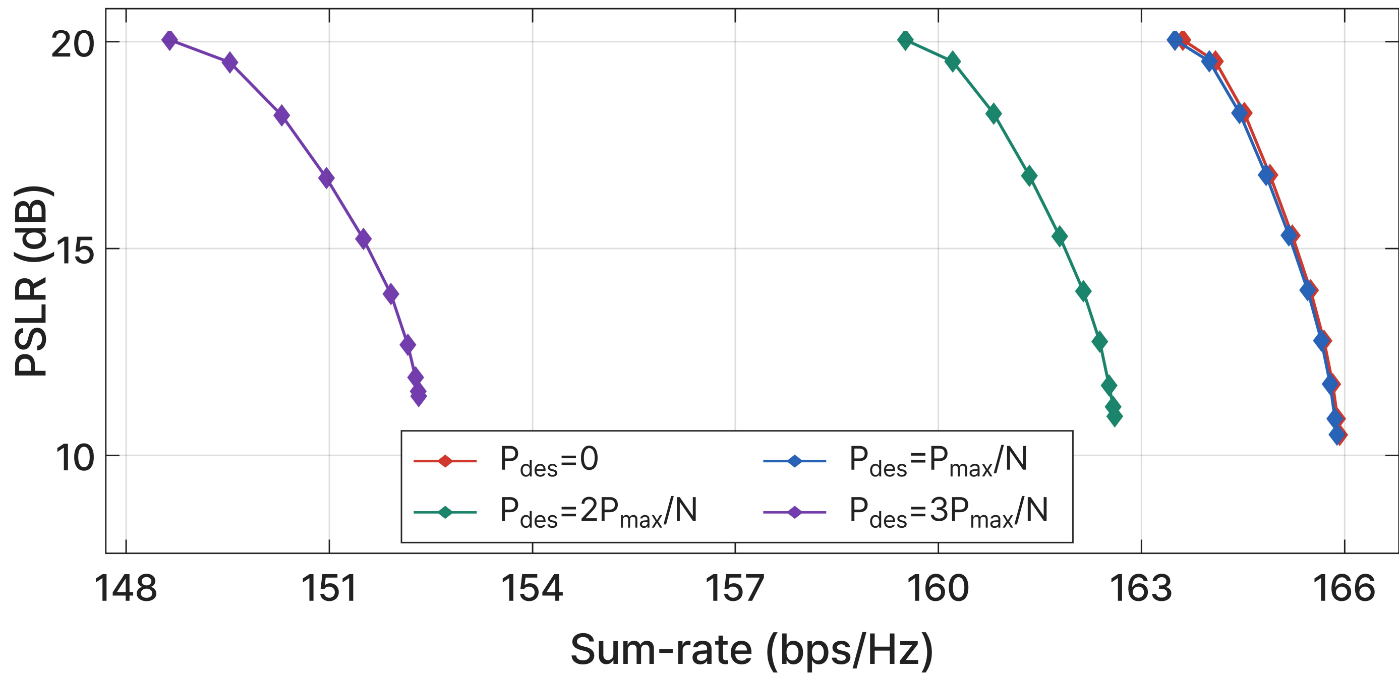
PSLR Pareto vs. P_{\text{des}}
