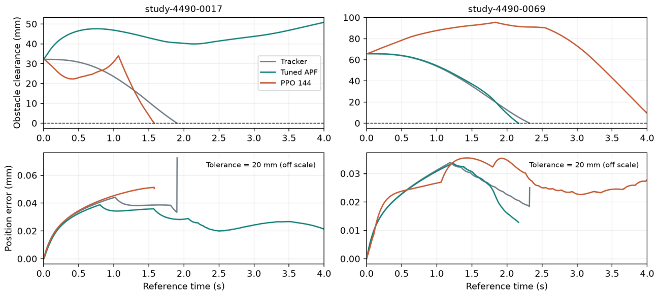
Figure 3. Two fixed-test examples. Lines end at actual termination; a missing suffix is not zero error. Dashed lines mark the 0.01 mm obstacle-contact band. The 20 mm tracking tolerance is off the error-plot scale. Geometry curves show sphere clearance; safety checks also include self-collision and limits.
