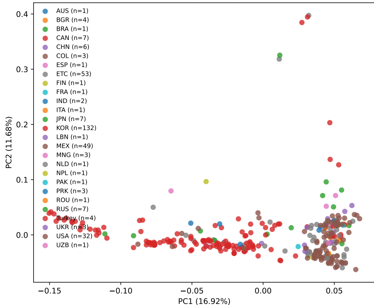
PCA by country
