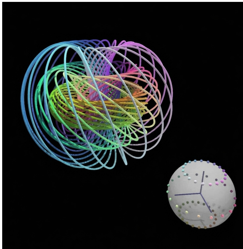
Figure 3: Figure 0.3 — Hopf fibration as a bundle. Source: Kingdom Come app/assets/home/hopf_fibration_bundle.png .
