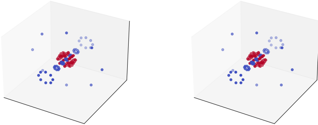
Figure 6.2: Figure 6.4 — Gauge equivalence of two flux topographs.
