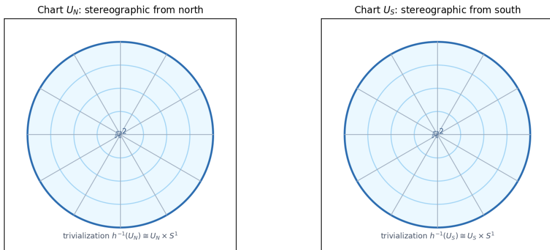
Figure 2.5: Auxiliary Figure A2.2 — Local charts on base S^2 .
