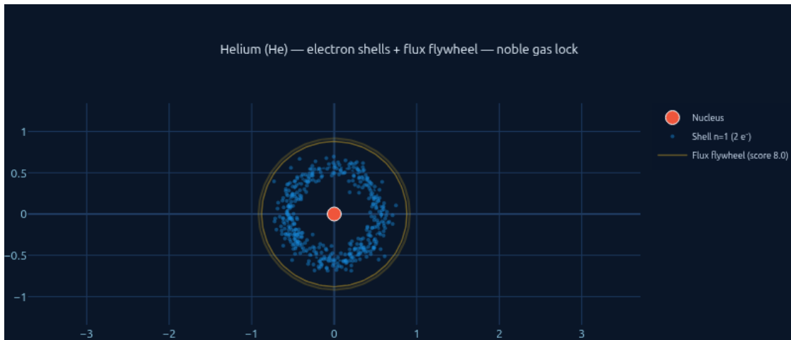
Figure 5: Auxiliary Figure A0.1 — Helium ( Z = 2 ) flux-flywheel still: closed-shell archetype with high model stability. Source: Kingdom Come z_knowns/frame_0002.png .
