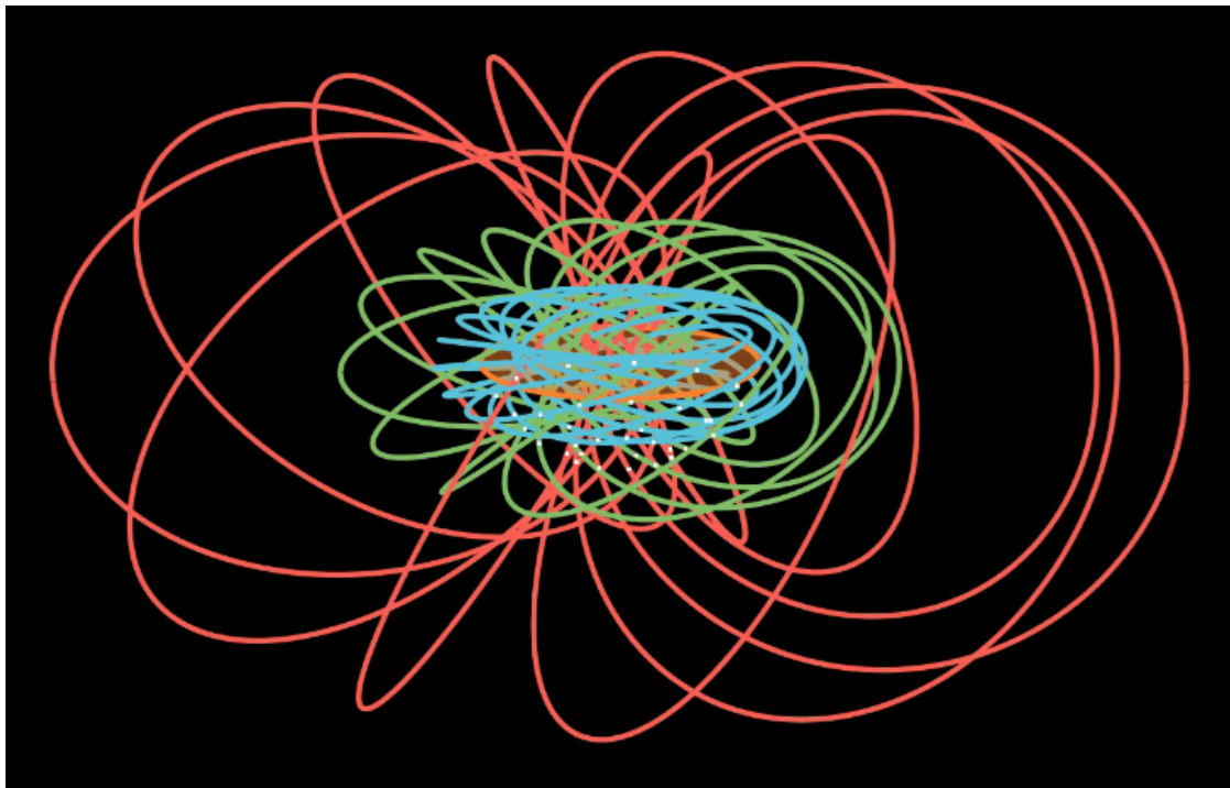
Figure 1: Figure 0.1 — Linked Hopf fibers (stereographic view). Source: Kingdom Come app/assets/home/hopf_linked_fibers.png .
