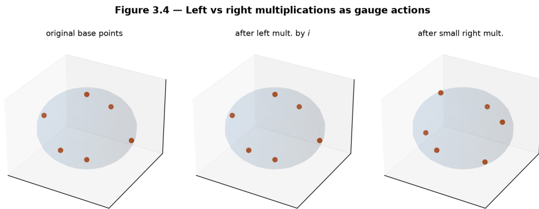
Figure 3.4: Figure 3.4 — Left vs right multiplications as gauge actions.
