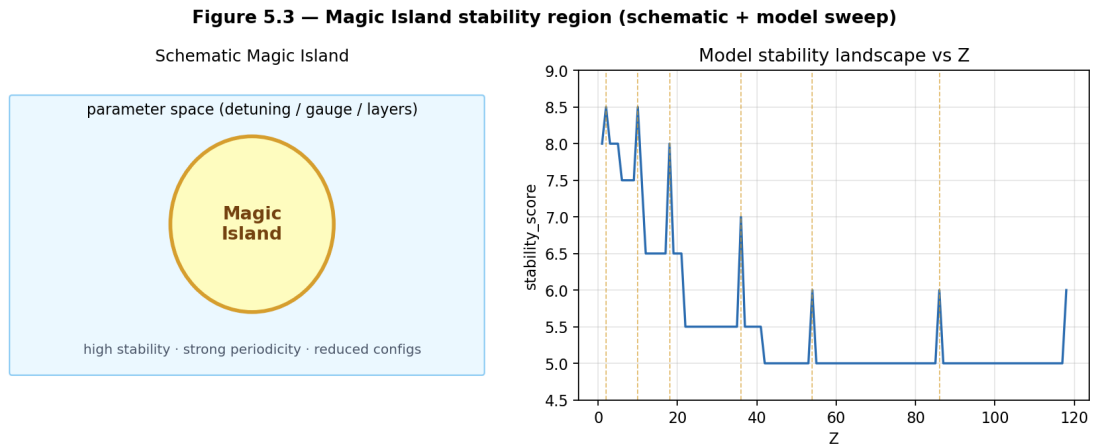
Figure 5.3: Figure 5.3 — Magic Island stability region.
