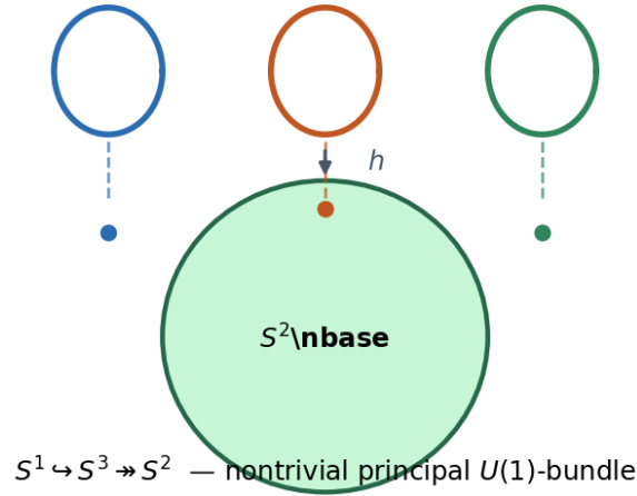
Figure 2.4: Figure 2.4 — Bundle picture: total space, fibers, base.
