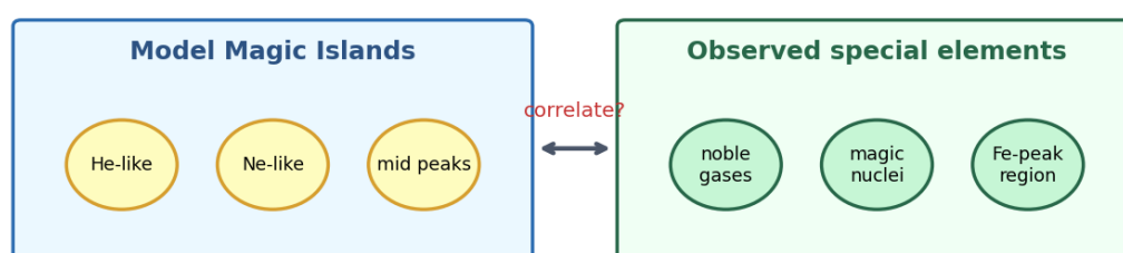
Figure 10.3 — Magic Island predictions vs observed specialness (schematic)
