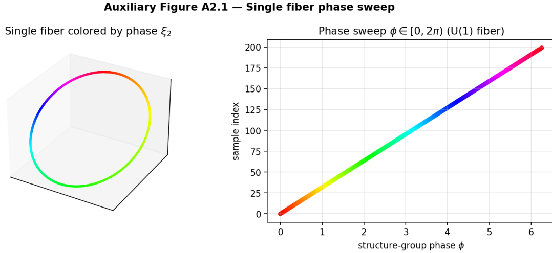
Figure 2.6: Auxiliary Figure A2.1 — Single fiber phase sweep.
