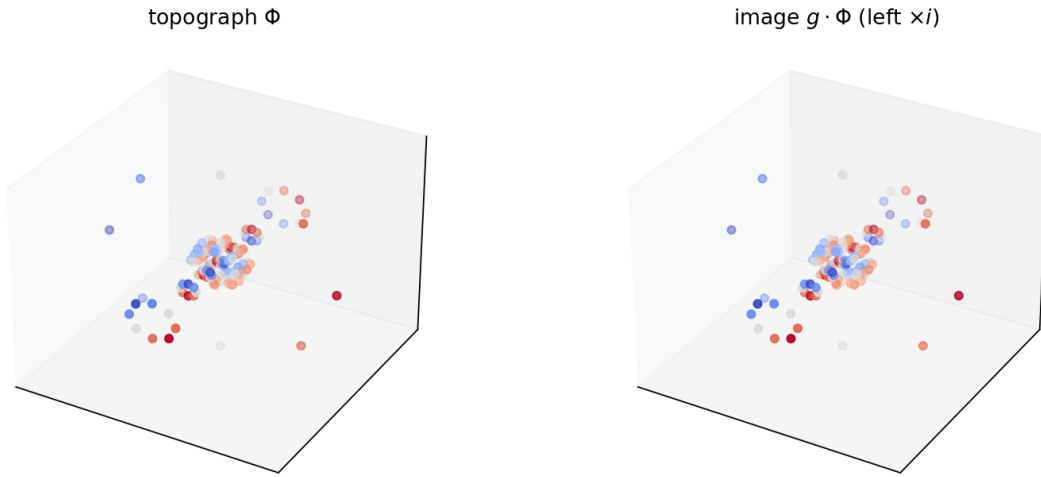
Figure 5.4 — Gauge symmetry acting on a flux topograph
