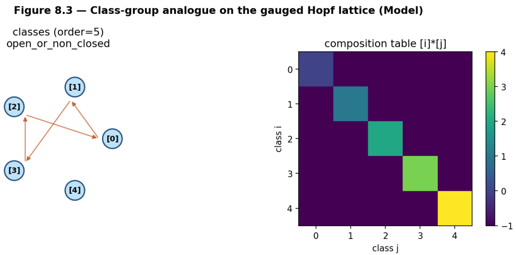
Figure 8.3: Figure 8.3 — Class-group analogue.
