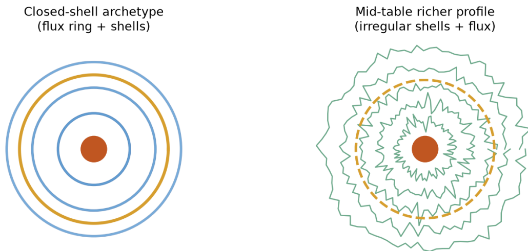
Figure 7.4: Figure 7.4 — Electron cloud as flux distribution (visual, not chemistry).
