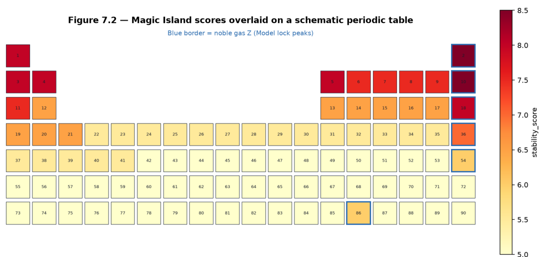
Figure 7.2: Figure 7.2 — Magic Island scores on a schematic periodic table.
